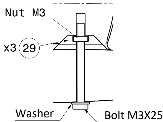
Detail Z
