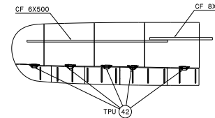
TAIL SECTION
