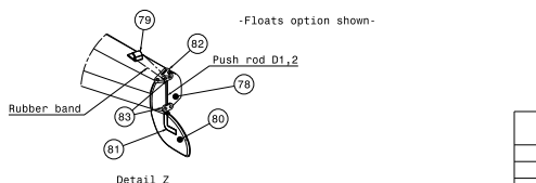
Detail Z
